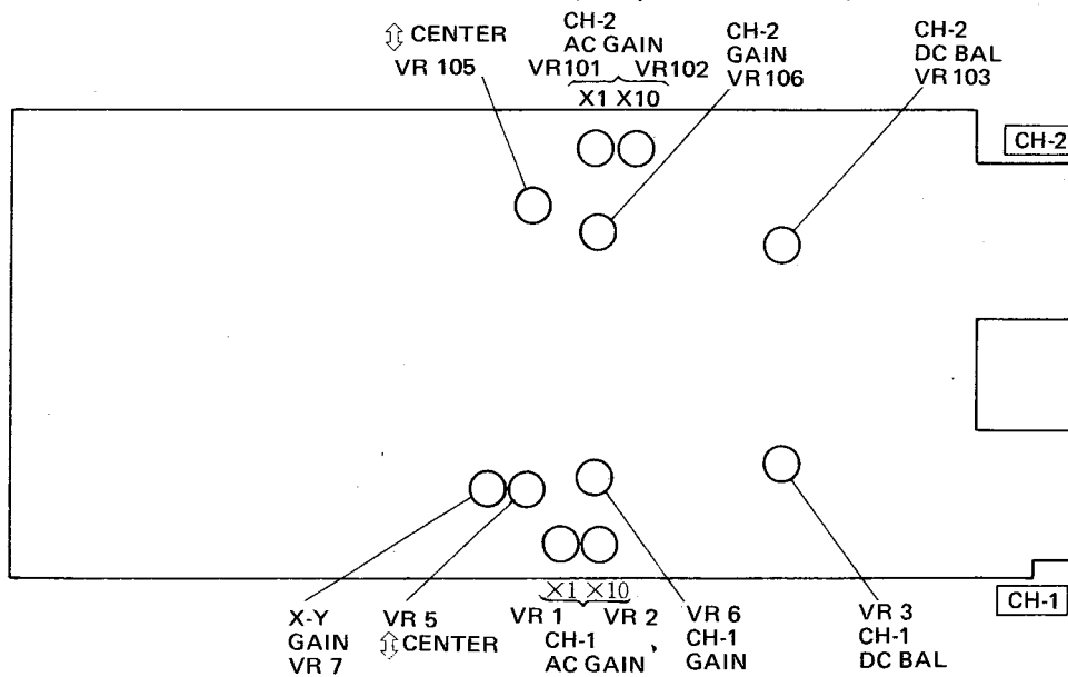
T-2554 V AMP PC-BOARD (Components side view)
